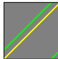
FIGURE 1. Level sets of the cost. Ensemble de niveau de c .
